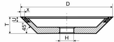
12V9-45° D*U*X*T*H
