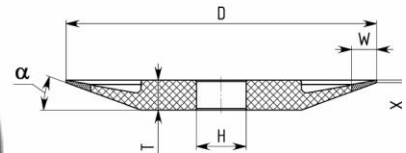
4BT9 D*T*X*W*H
