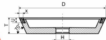
11V9-70° D*U*X*T*H
