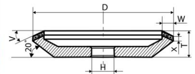
12V5-20 D*T*W*X*V*H
